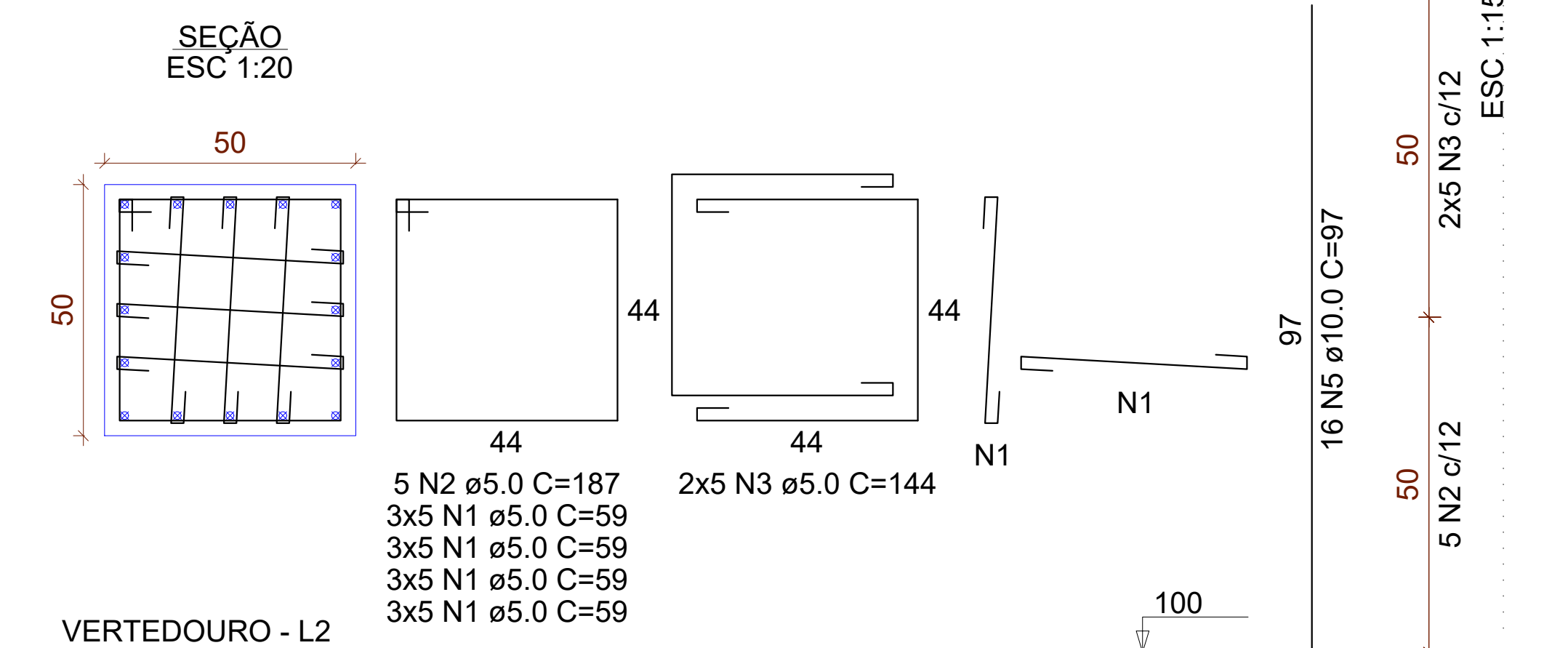
P11=P12=P13=P14=P15 VERTEDOURO TOPO - L3
