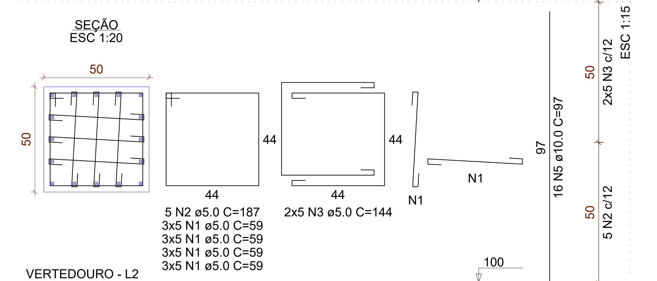
P11=P12=P13=P14=P15 VERTEDOURO TOPO - L3
